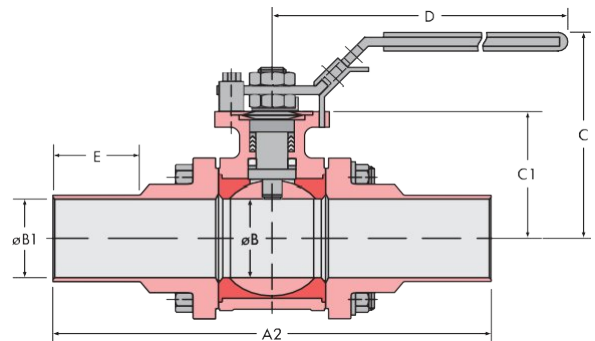
Extended Tube End Connections Model S7700
