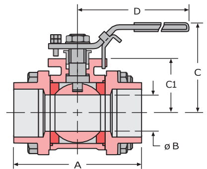
Socket Weld End
