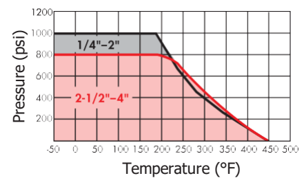
PRESSURE/TEMPERATURE - RPTFE Seat Material
